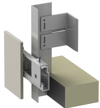
DETAIL: ALPHA VCI.40 SUBFRAMING
