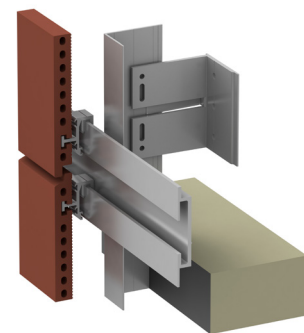
DETAIL: ALPHA VCI.45 SUBFRAMING SYSTEM
